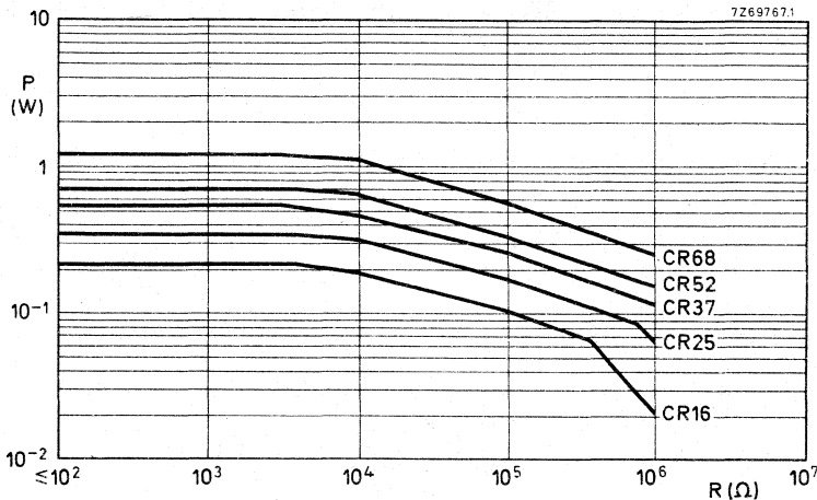
Fig. 4 Maximum permissible dissipation at T_{amb} = 70\text{ °C} as a function of the resistance value for a resistance drift of 1,5% after 1000 hours or for a maximum temperature of 155 °C without reaching the resistance drift of 1,5%, limiting voltage being taken into account.
