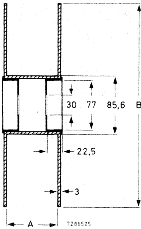
Fig. 9 Reel dimensions.
