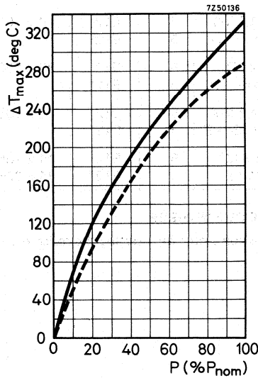
Fig. 4 Maximum temperature rise as a function of the dissipation. The dotted line refers to mounting with bolt and metal plate.
